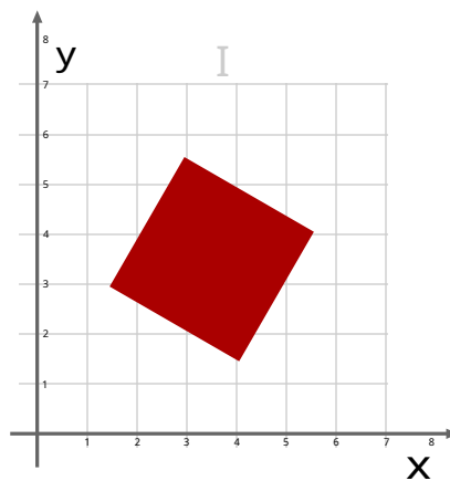
Figure 18: The result of applying a rotation matrix
